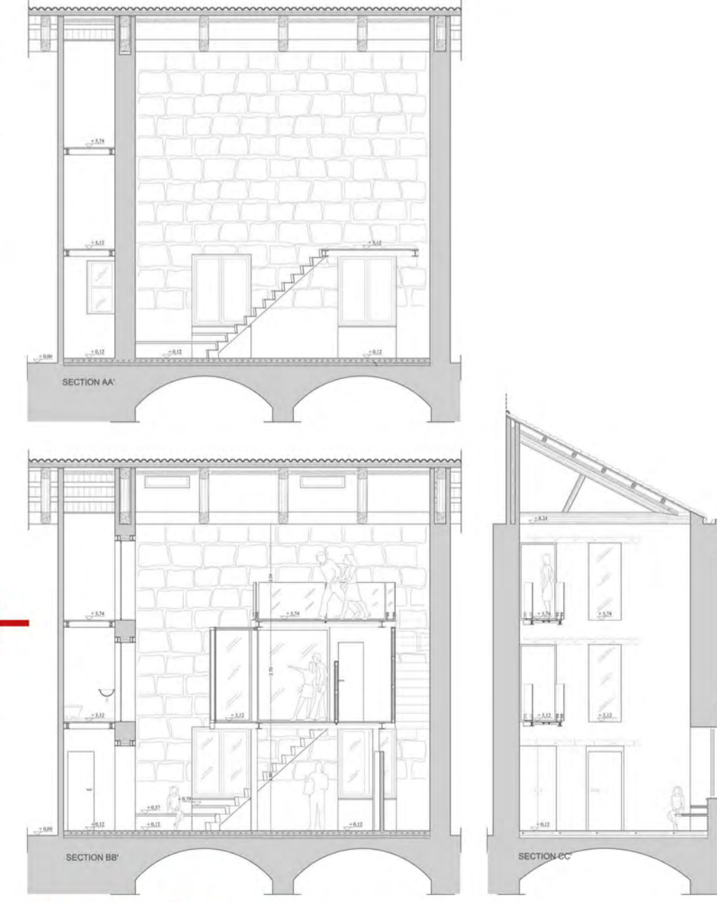
SECTIONS
