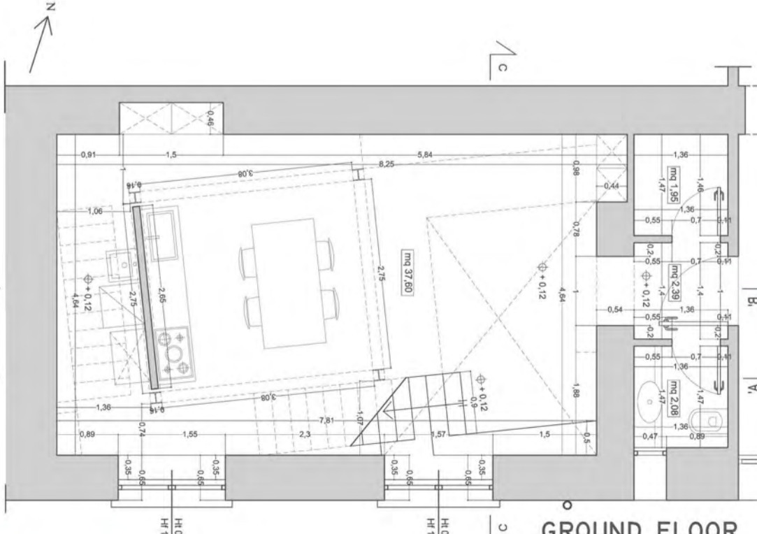
PLANS
